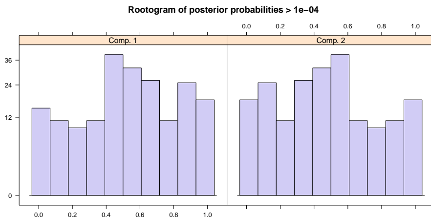
Figure 3: plot(m2)
