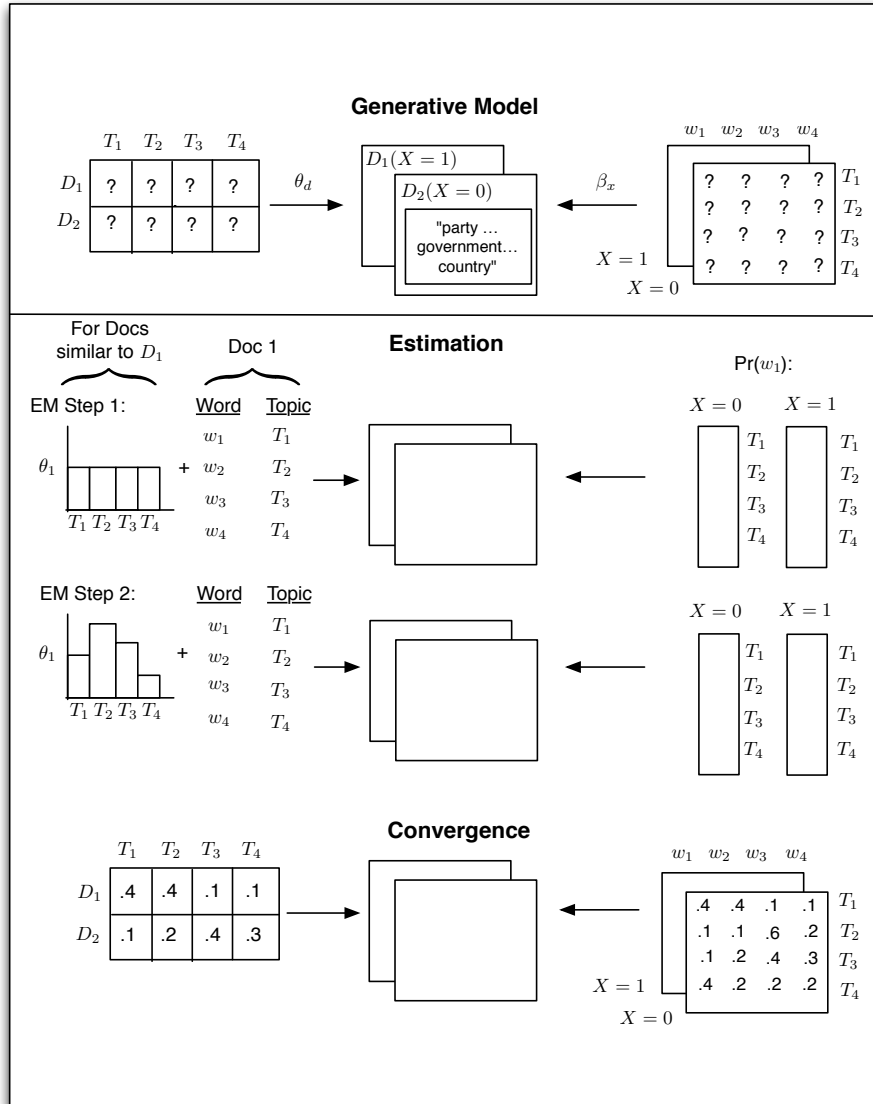
Figure 1: Heuristic description of generative process and estimation of STM.
