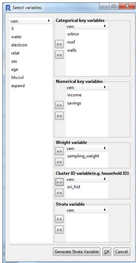
Figure 3: The variable selection frame of the GUI.
