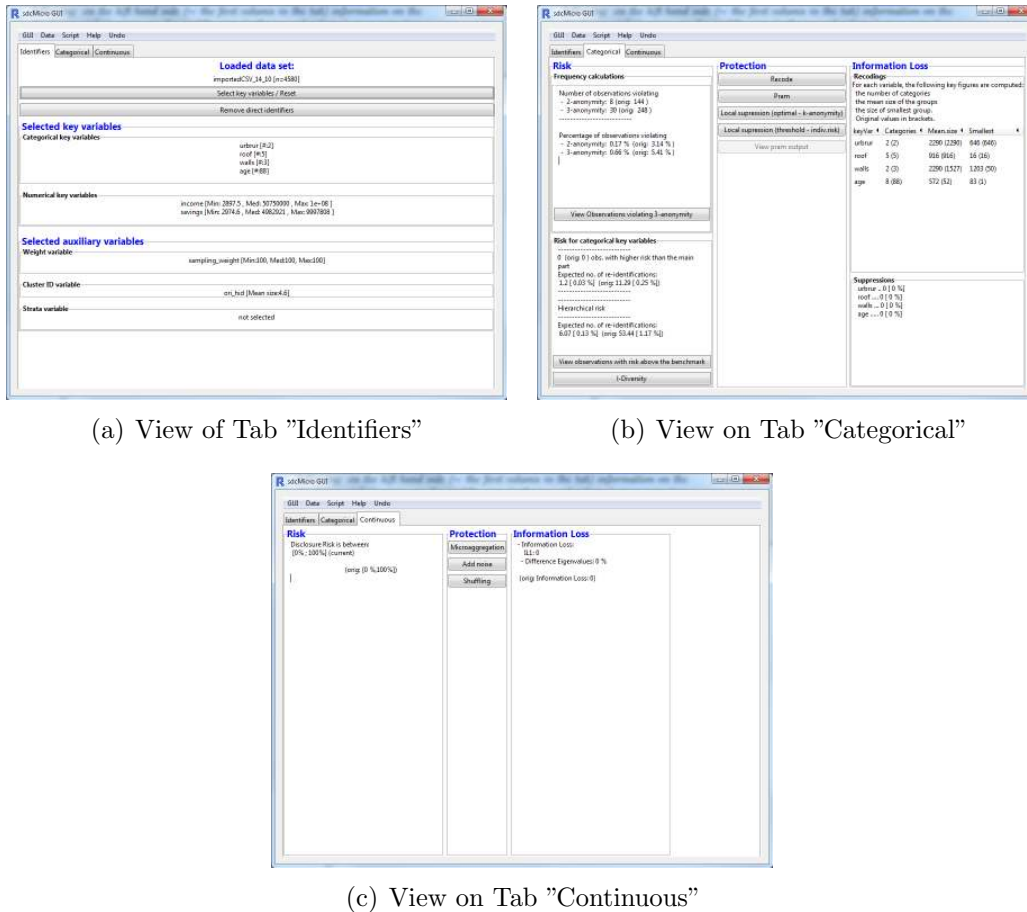
Figure 5: Showing the three main tabs of the GUI. Information on the content was already given in 1.1.
