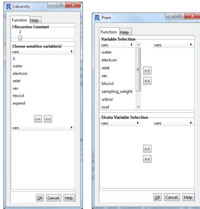
(a) l -Diversity. (b) Post randomization method (PRAM).
