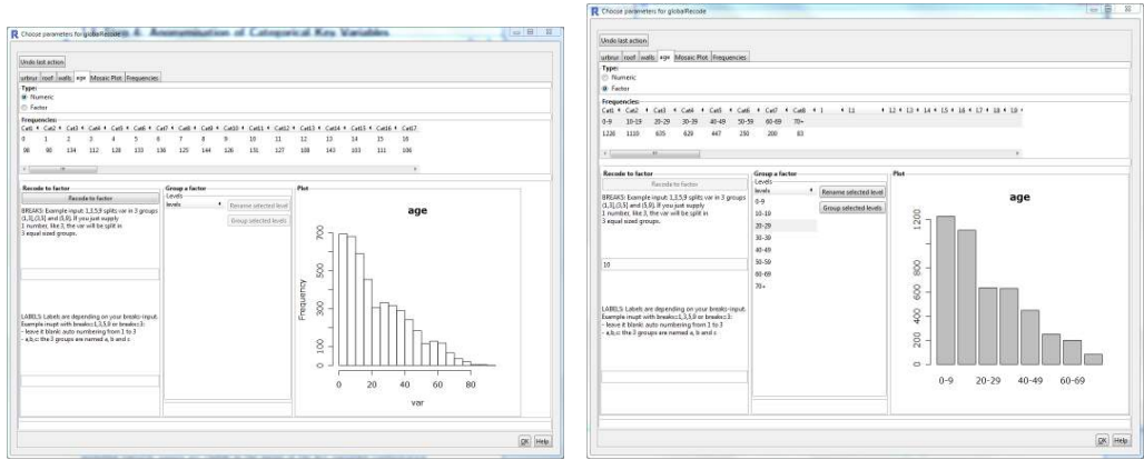
(a) Original distribution of age (continuous). (b) Variable age recoded into age groups and converted to a factor.
