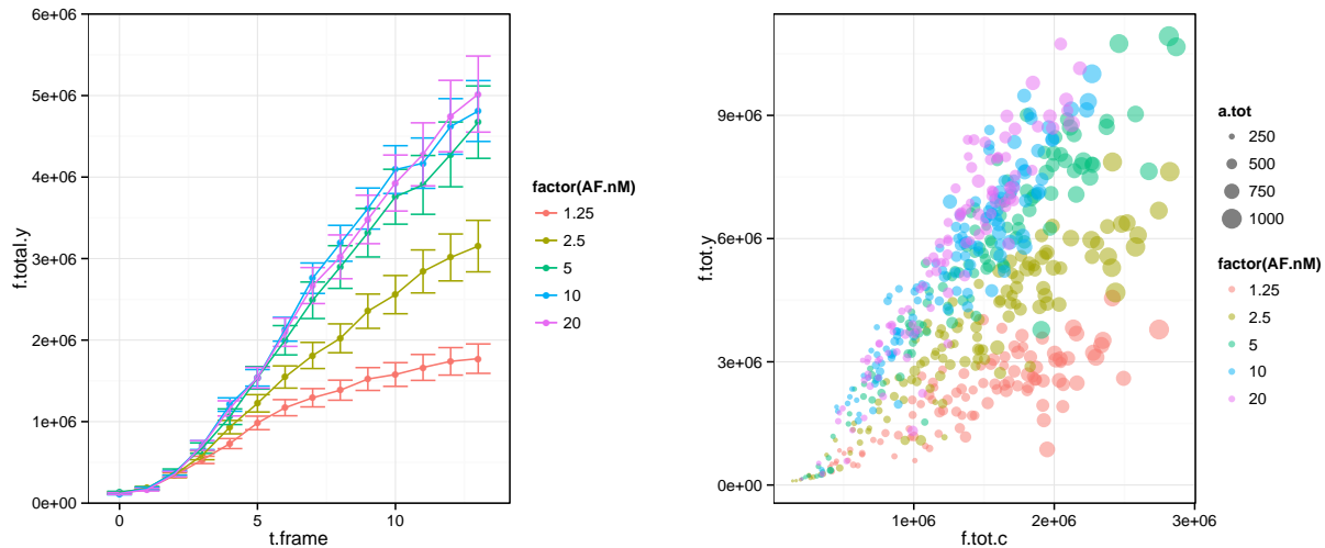
Figure 6: Left: Mean YFP total fluorescence ( f.total.y ) vs time ( t.frame ) for different doses of pheromone ( AF.nM ). Right: Scatter plot of YFP vs CFP fluorescence, colored by AF.nM and size proportional to cell area.
