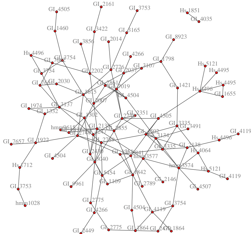
Figure 11: The inferred graph for human gene expression data using Gaussian copula graphical models. This graph consists of links with estimated posterior probabilities greater than 0.995.
