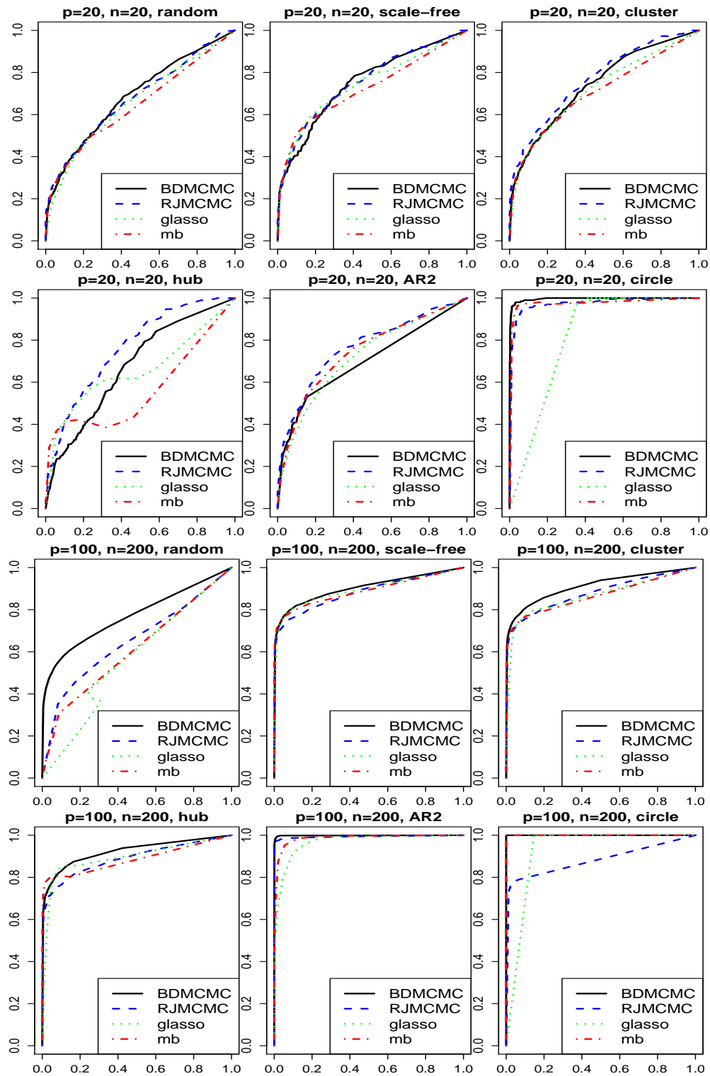
Figure 7: ROC curves present the performances of the two sampling algorithms from the BDgraph package and two frequentist methods from the huge package for p = \{20, 100\} and varying graph structures and with with 50 replications.
