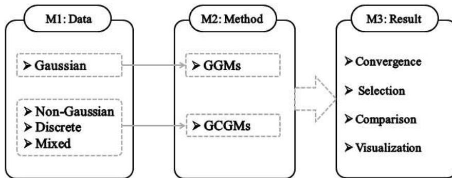
Figure 1: Configuration of the BDgraph package which includes three main parts: (M1) data generation, (M2) several search algorithms, (M3) various functions to evaluate convergence of the search algorithms, estimation of the true graph, assessment and comparison of the results and graph visualization.
