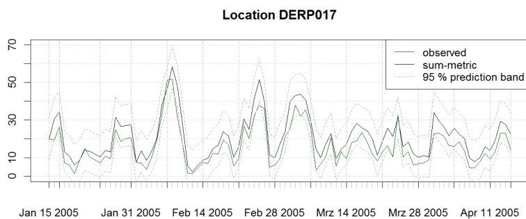
Figure 5: Subset of the time series of observed and predicted \text{PM}_{10} at a single station in Lower Saxony along with its 95 % prediction intervals.
