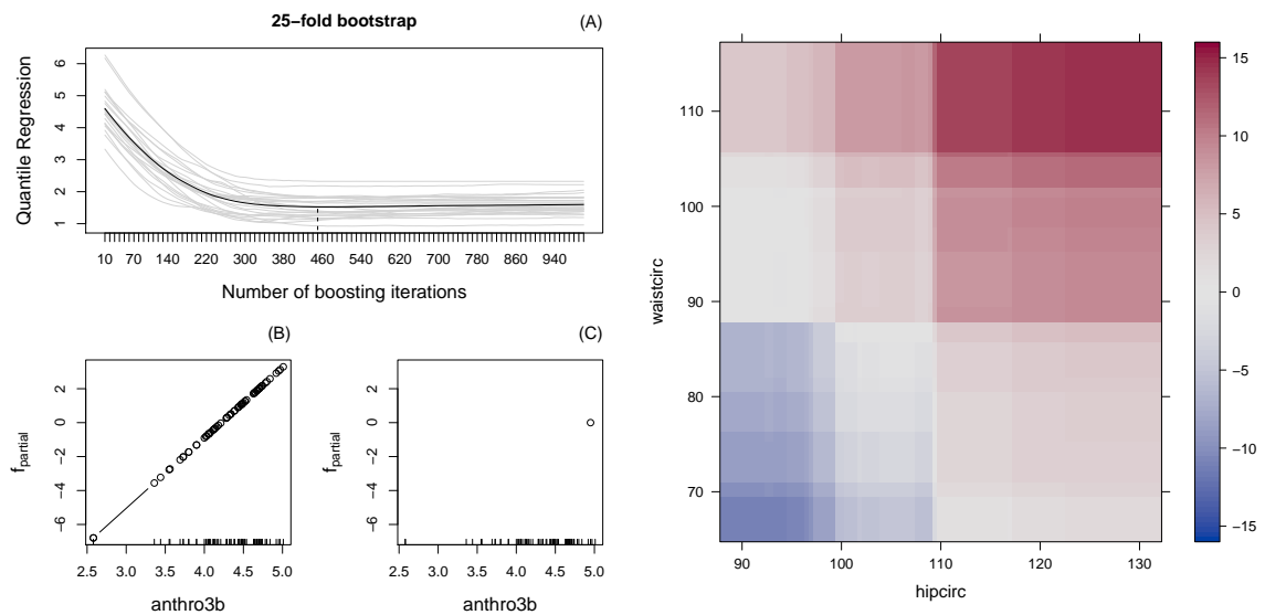
Figure 1: Out-of-bag empirical risk (A) indicating that 450 iterations are appropriate. Fitted model components for variable anthro3b , consisting of a linear (B) and smooth term (C). The right panel shows the interaction model component between hip and waist circumferences.
