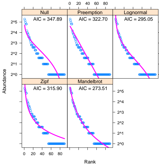
Figure 4: Ranked abundance distribution models for a random plot (no. 3). The best model has the lowest AIC.
