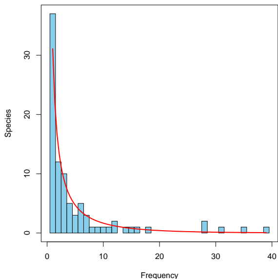
Figure 3: Fisher’s log-series fitted to one randomly selected site (3).
