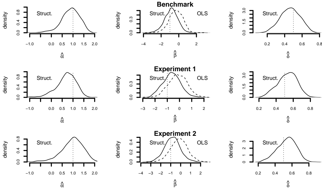
Figure 5: Posterior distributions of parameters for benchmark simulations. True value are given by vertical, dotted lines. Structural model and OLS estimates for 1,000 draws are given by straight and dashed lines, respectively.
