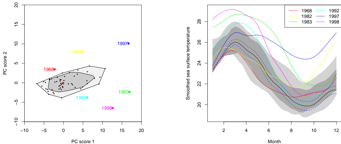
(a) The bivariate bagplot.
