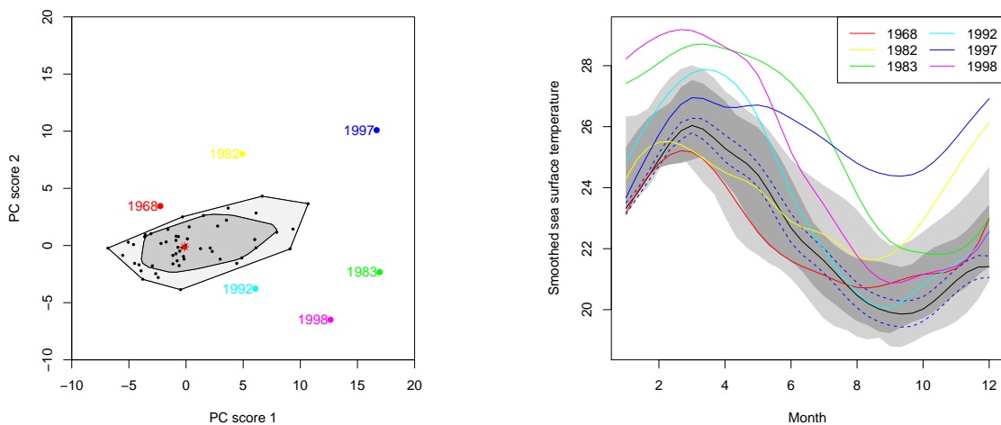
(a) The bivariate HDR boxplot.
