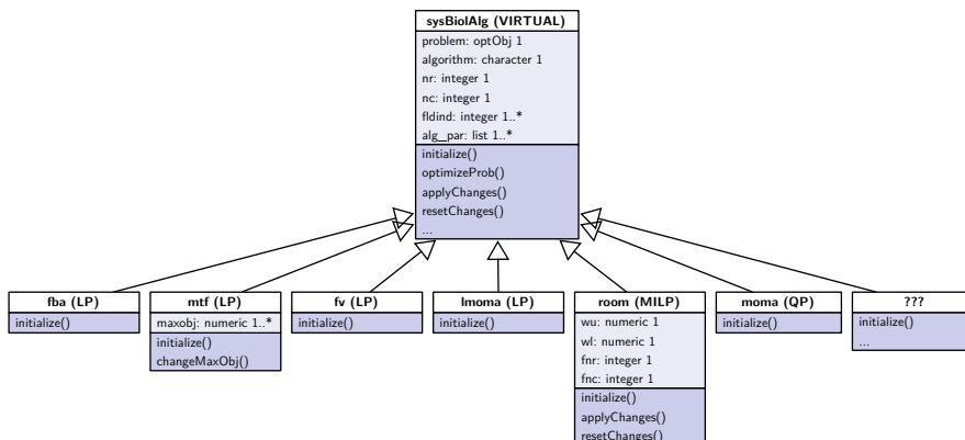
Figure 5: UML representation of class sysBio1Alg .
