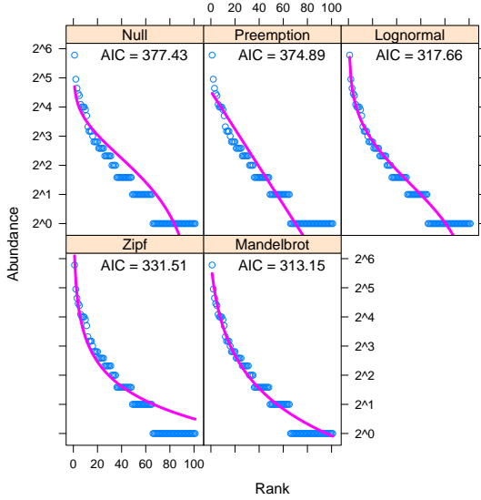
Figure 4: Ranked abundance distribution models for a random plot (no. 5). The best model has the lowest AIC.
