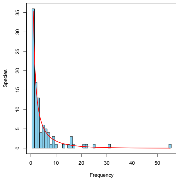
Figure 3: Fisher's log-series fitted to one randomly selected site (5).
