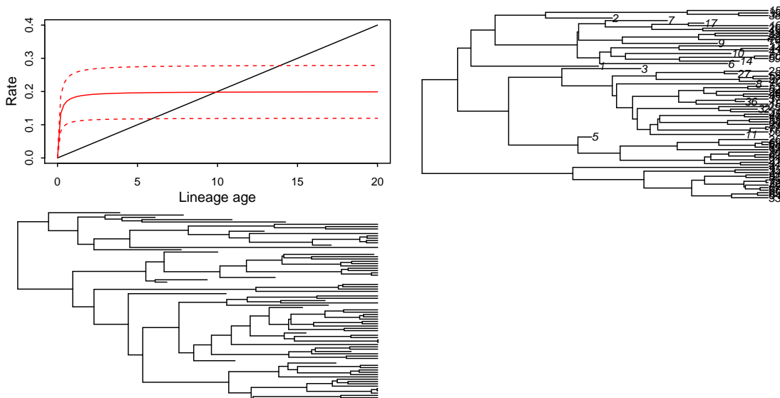
Figure 16: Simulations using expressions. a) Simulated extinction and speciation rates. Extinction (black) shows senescence and speciation shows latency. For the first simulation (b: latencyTree ), speciation is determined entirely by lineage age and there are relatively few extant basal species and few rapid sequences of speciation along branches. For the second (c: latTraitTree ), there are again few rapid sequence of speciation and simulated body mass (red bars) is predominantly smaller than the ancestral average (width of the grey bar). The dashed red lines in a) show the speciation rate for species with simulated log body mass 2 units higher and lower than the ancestral mean.
