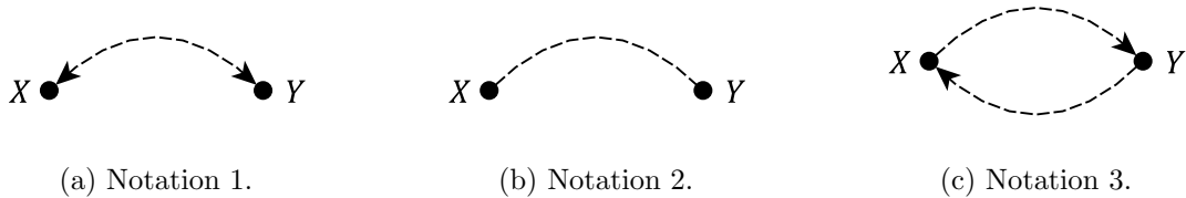
Figure 6: Notations for bidirected edges.
