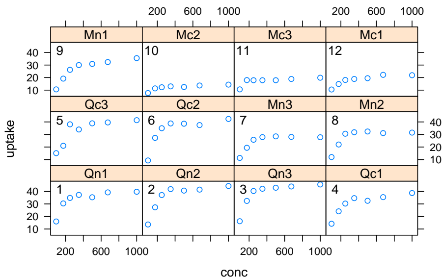
Figure 1: fn$xyplot
