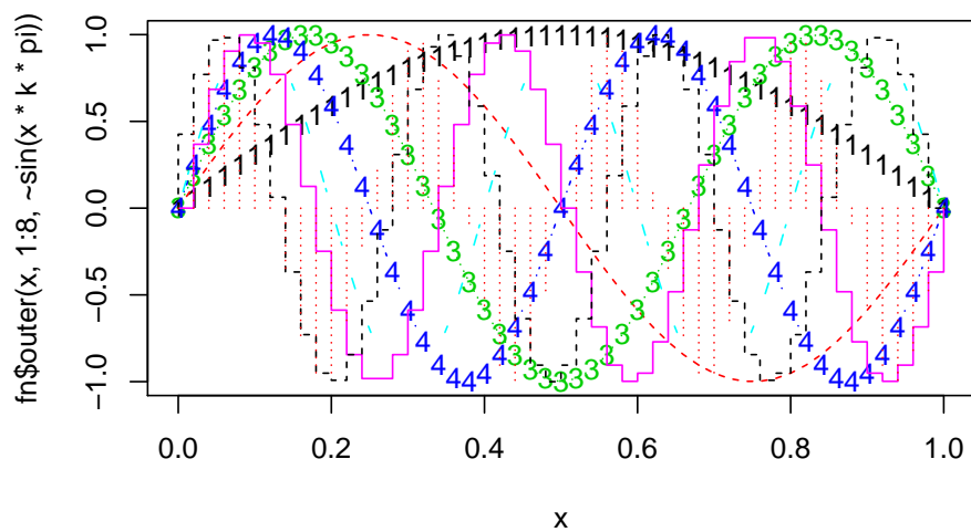
Figure 3: matplot(x, fn$out(x, 1:8, ~ sin(x * k*pi)), type = 'blobcsSh')
