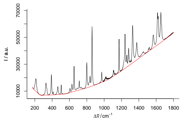
(a) Bent paracetamol spectrum and rubberband baseline.
