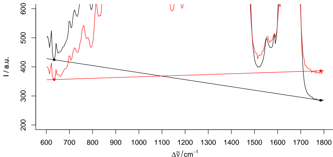
Figure 1 Fitting a linear baseline through two points. If the signal to noise ratio is not ideal, wavenumbers that work fine for one spectrum (black) may not be appropriate for another (red).
