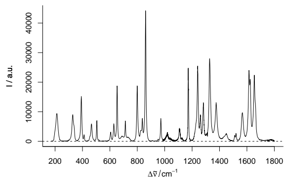
(b) Corrected spectrum.
