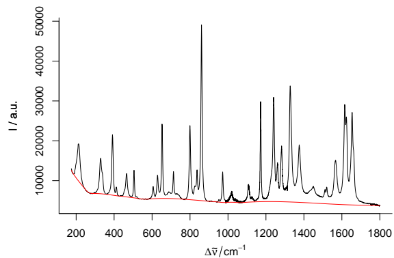
(a) paracetamol with the rubberband fitted baseline.
