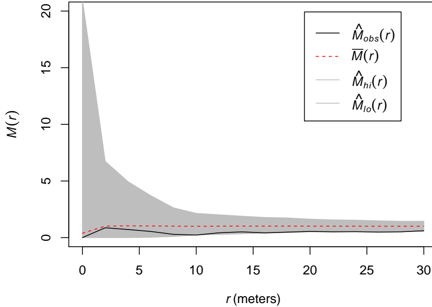
Figure 4. Representation of M(r) values of Qualea rosea around Vouacapoua Americana trees in the paracou16 point pattern. The solid, black curve is M . The dotted red curve is the average simulated value. The shaded area is the confidence envelope. M = 1 is expected if points are independently distributed. The risk level is 5%, 1000 simulations have been run. Distances are in meters.
