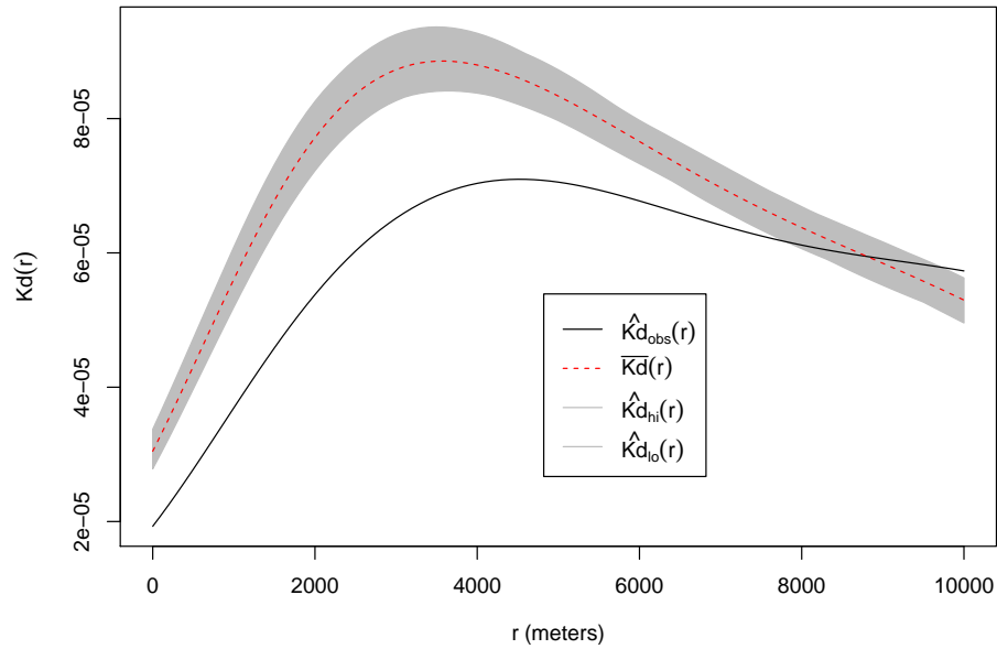
Figure 2. Representation of K_d(r) values of the 10% most serious emergencies in year 2004 in Toulouse urban area, showing their significant dispersion at all distances up to 10 km. The solid, black curve is K_d . The dotted red curve is the average simulated value and the shaded area is the confidence envelope under the null hypothesis of random location. The risk level is 5%, 1000 simulations have been run. Distances are in meters.
