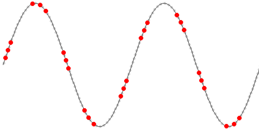
Fig. 5. Detectors placed with make.line
