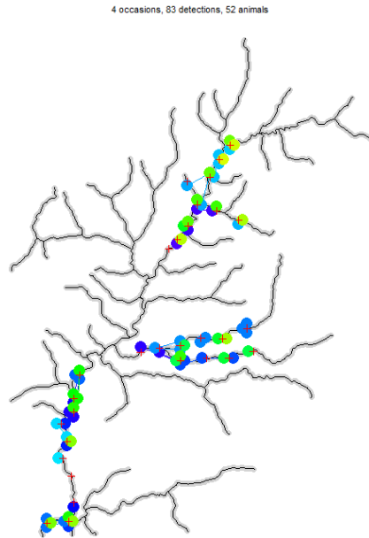
Fig. 6. Simulated detections of linear population. Colours vary (subtly) among individuals. Red crosses indicate trap locations. Movements ('tracks') are shown as-the-crow-flies rather than along the network.
