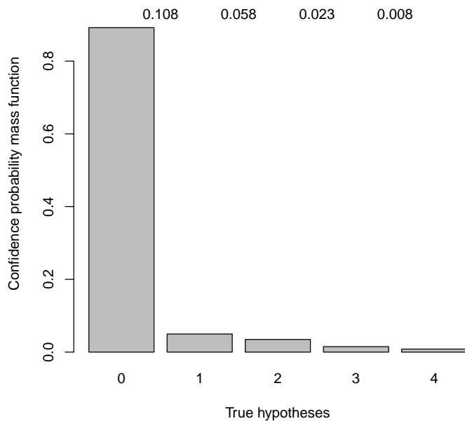
Figure 1: pick(cta, names(ps), plot=TRUE)
