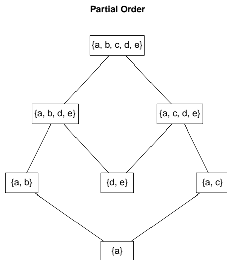
Figure 1: Knowledge Structure
