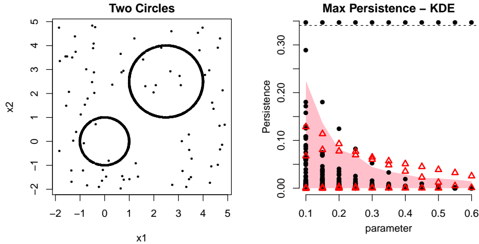
Figure 11: Max Persistence Method for the selection of smoothing parameters. For each value of the smoothing parameter we display the persistence of the corresponding homological features, along with a (pink) confidence band that separates the statistically significant features from the topological noise.
