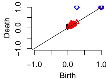
Figure 7: Persistence diagram of Alpha shape. Black points represent connected components, red triangles represent loops, and blue diamonds represent voids.
