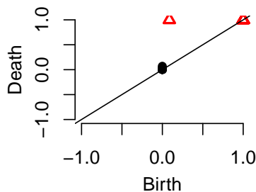
Figure 6: Persistence diagram of Alpha complex. Black points represent connected components and red triangles represent loops.
