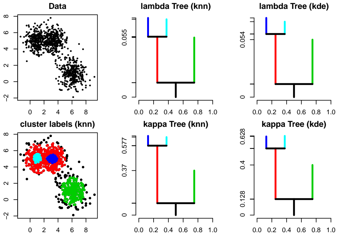
Figure 12: The lambda trees and kappa trees of the k Nearest Neighbor density estimator and the kernel density estimator.
