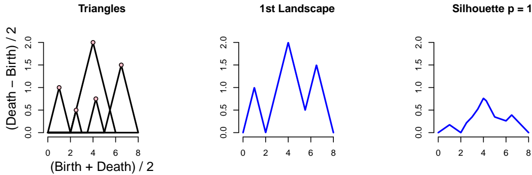
Figure 8: Left: we use the rotated axes to represent a persistence diagram D . A feature (b, d) \in D is represented by the point (\frac{b+d}{2}, \frac{d-b}{2}) (pink). In words, the x -coordinate is the average parameter value over which the feature exists, and the y -coordinate is the half-life of the feature. Middle: the blue curve is the landscape \lambda(1, \cdot) . Right: the blue curve is the silhouette \phi^{(1)}(\cdot) .
