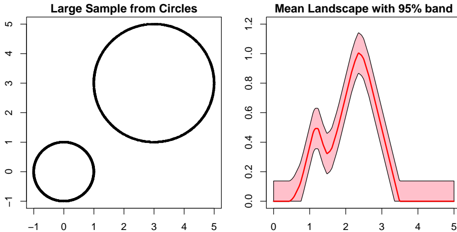
Figure 10: 95% confidence band for the mean landscape function.
