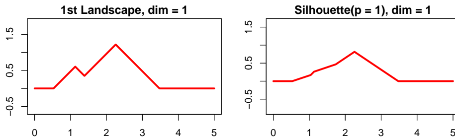
Figure 9: Landscape and Silhouette of the one-dimensional features of the diagram of Figure 5.
