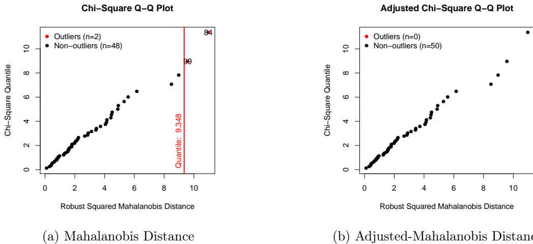
Figure 4: Multivariate outlier detection.
