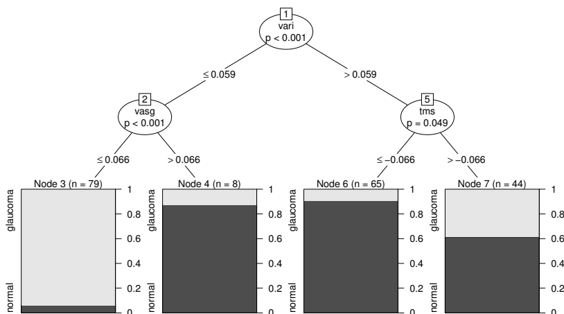
Figure 8.5 Glaucoma data: Conditional inference tree with the distribution of glaucomateous eyes shown for each terminal leaf.
