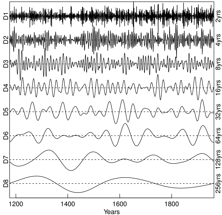
Figure 6: Multiresolution analysis of the Mesa Verde chronology
