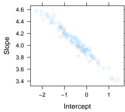
B: 100 simulations
