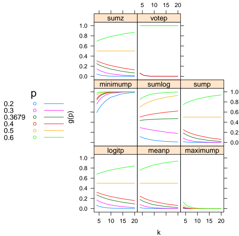
Figure 2: Behaviour of the methods for k values of p = p_i
