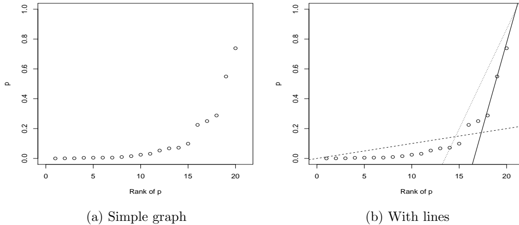
Figure 1: Ouput from schweder
