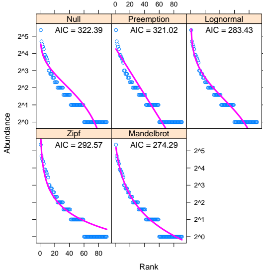
Figure 4: Ranked abundance distribution models for a random plot (no. 48). The best model has the lowest AIC.
