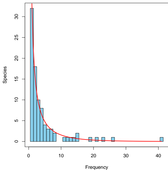
Figure 3: Fisher’s log-series fitted to one randomly selected site (48).
