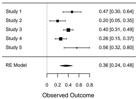
Multivariate meta-analysis
