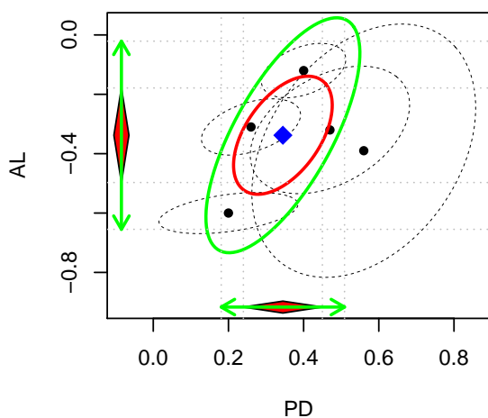
Multivariate meta-analysis
