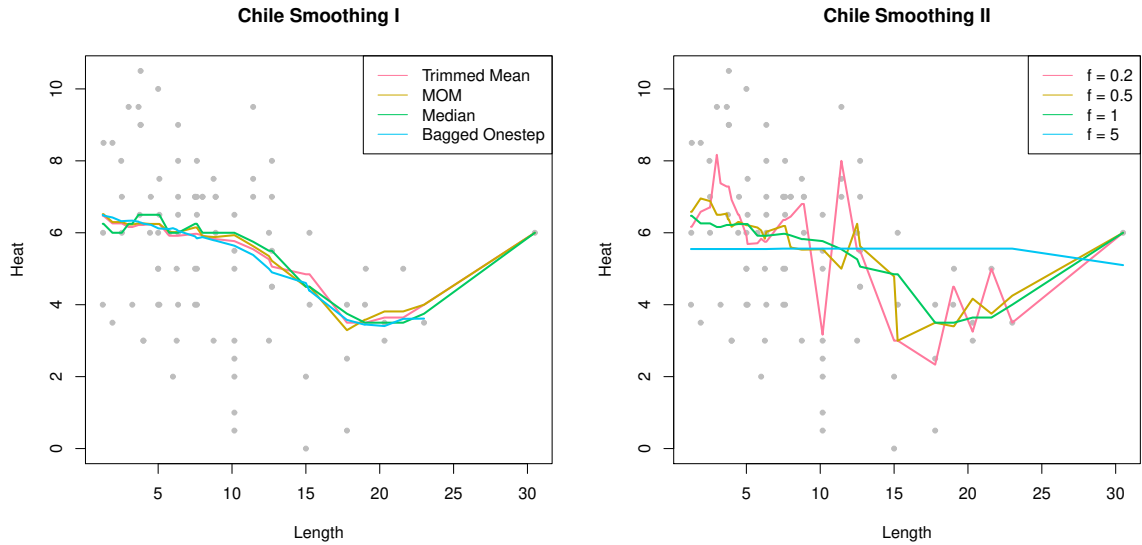
Figure 7: Left panel: smoothers with various robust location measures. Right panel: trimmed mean smoother with varying smoothing parameter f .
