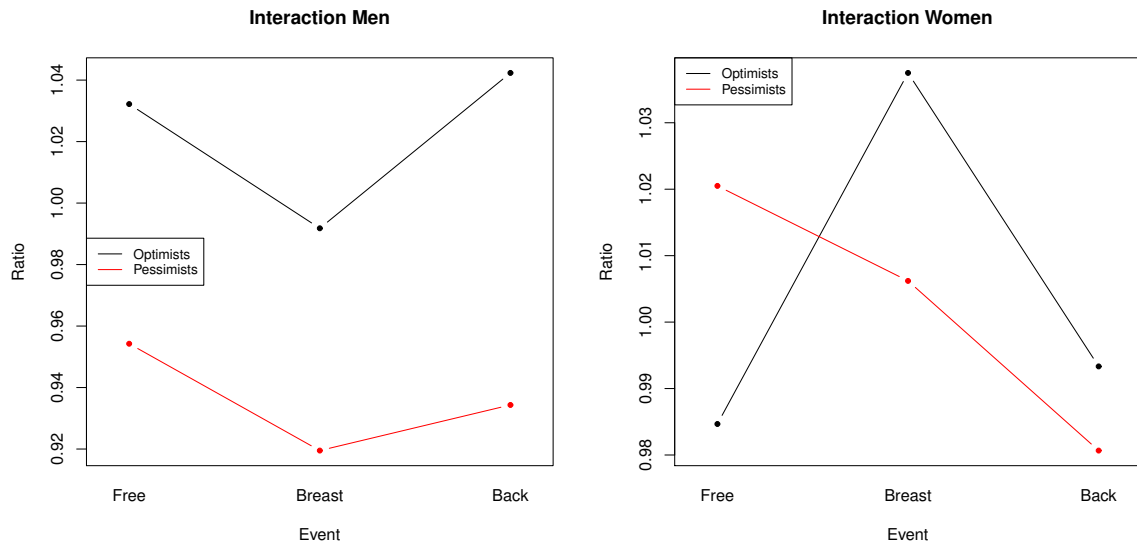
Figure 5: Interaction plot involving the trimmed means of the time ratio response for males and females separately.
