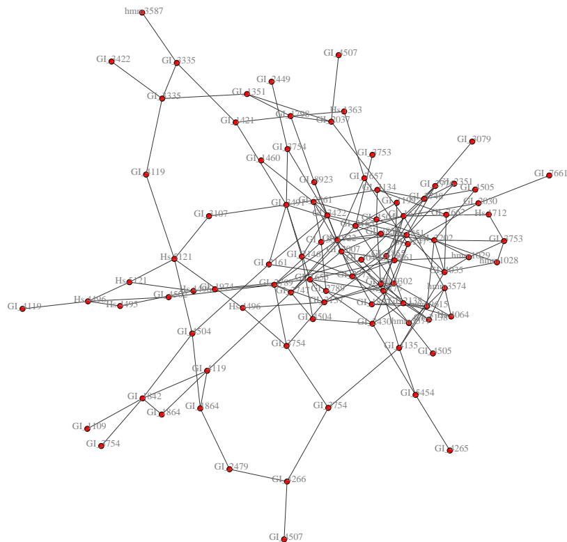
Figure 9: The inferred graph for human gene expression data using Gaussian copula graphical models. This graph consists of 176 links with estimated posterior probabilities greater than 0.5.
