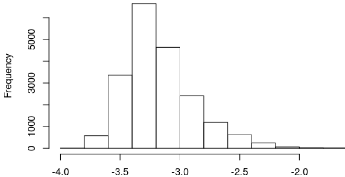
Histogram of log10 of Hat values
