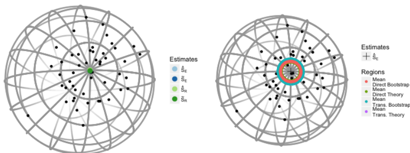
Figure 1: The x -axis of a random sample from the Cayley-UARS distribution with \kappa = 1 , n = 50 . All for point estimates are displayed on the left and all three region methods along with the projected mean are on the right.
