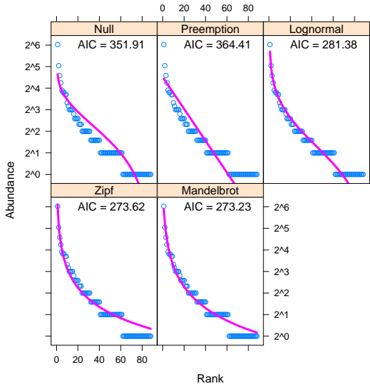
Figure 4: Ranked abundance distribution models for a random plot (no. 37). The best model has the lowest AIC.
