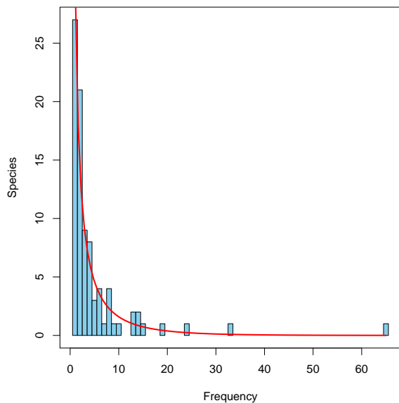
Figure 3: Fisher’s log-series fitted to one randomly selected site (37).
