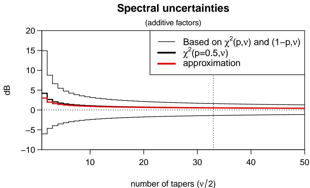
Figure 8: Additive spectral uncertainties by number of tapers needed to create 95% confidence intervals. These quantized curves are found by evaluating the \chi^2 distribution, where \nu is the number of degrees of freedom (two per taper). The thick, red line shows an approximation to these uncertainties based on 1/\sqrt{\nu-1} , which is accurate to within a few percent in most cases. The vertical dotted-line shows the number of tapers need to make the width less than 3 decibels.
