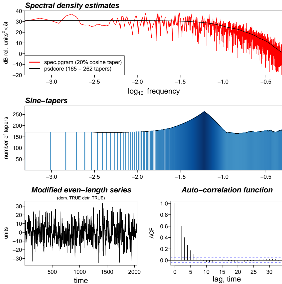
Figure 2: A summary plot produced by psdcore when plot=TRUE. Top: Comparison between PSD estimators for the cleaned Project MAGNET data. The frequency axis is in units of log 10 km -1 , and power axis is in decibels. Middle: The number of tapers applied as a function of frequency from the plot.tapers method. Bottom: The spatial series used to estimate the PSDs and a subset of the full autocorrelation function.
