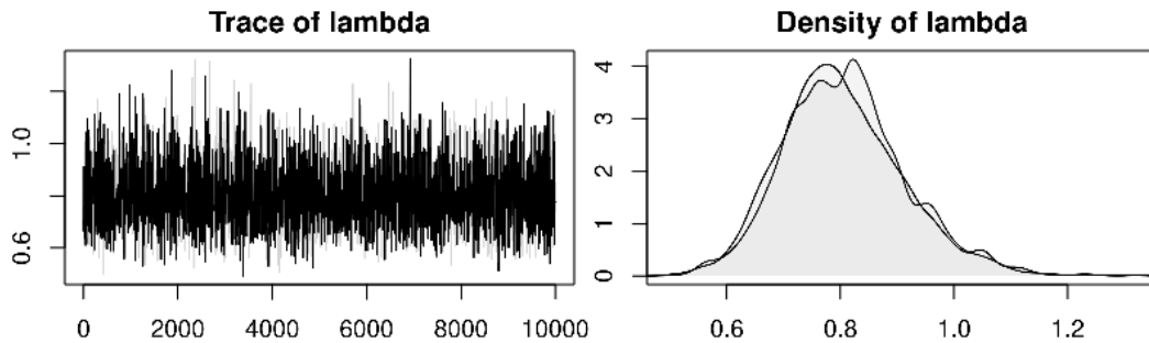
Figure 8: Plot of \lambda , the key hyperparameter of the Minnesota prior, for separate runs.
