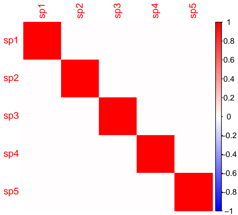
Figure 5: Heatmap of the Omega matrix
