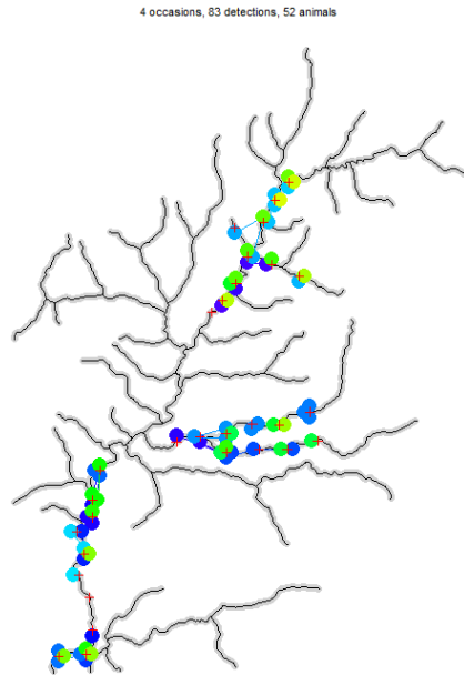
Fig. 6. Simulated detections of linear population. Colours vary (subtly) among individuals. Red crosses indicate trap locations. Movements ('tracks') are shown as-the-crow-flies rather than along the network.
